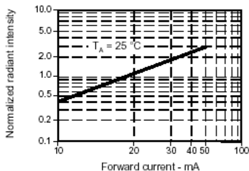
Fig. 2 Radiant Intensity vs Forward Current gra_028.ds4
