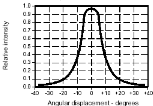
Fig. 1 Radiant Intensity vs Angular Displacement gra_027.ds4
