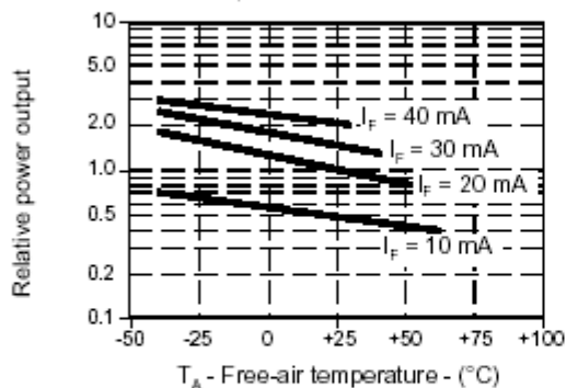
Fig. 7 Relative Power Output vs Free Air Temperature gra_130.ds4
